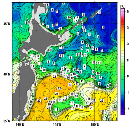
Daily 100m temperatures 15 Nov. 2023.
