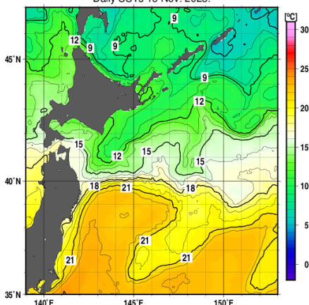
Daily SSTs 15 Nov. 2023.
